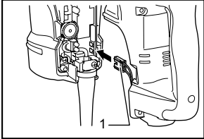
1. Connector
