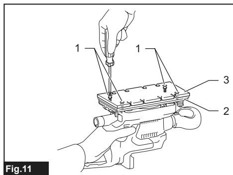
Fig. 11 ► 1. Screws 2. Sanding base 3. Pad
