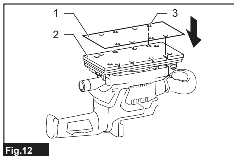
Fig. 12 ► 1. Abrasive paper 2. Pad 3. Dust-suction holes
